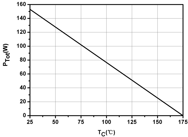
Fig.5-Power Derating
